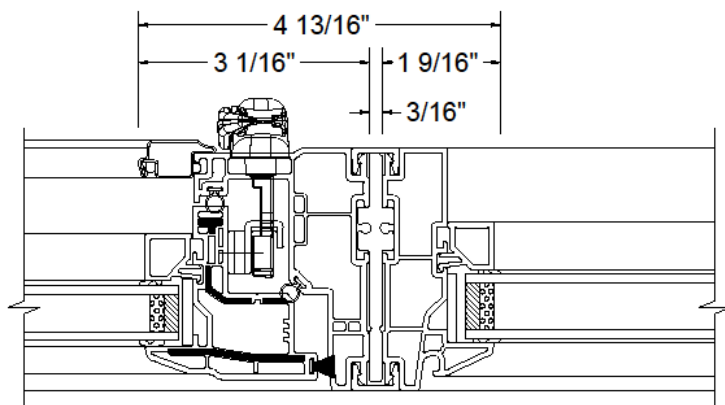
C - AWNING/FIXED(NO SASH) MULLION 3/16" REINFORCEMENT DETAIL
