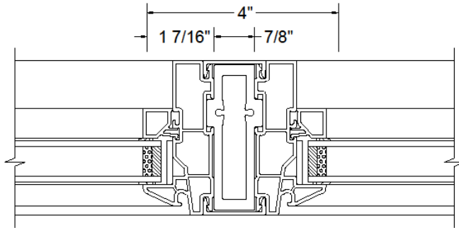
B - FIXED(NO SASH)/FIXED(NO SASH) MULLION 7/8" REINFORCEMENT DETAIL
