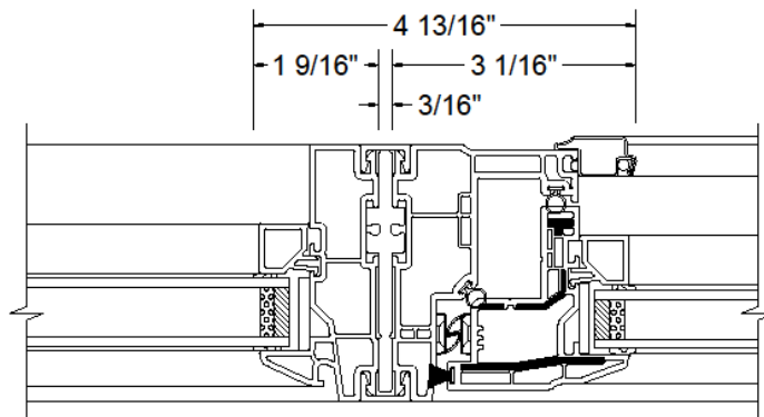
C - FIXED(NO SASH)/CASEMENT MULLION 3/16" REINFORCEMENT DETAIL
