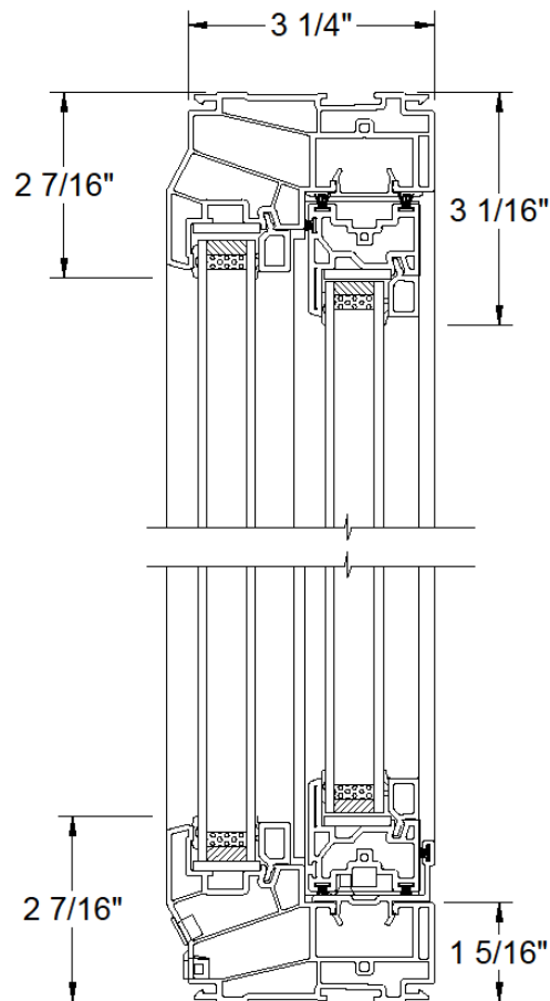
VERTICAL SECTION
