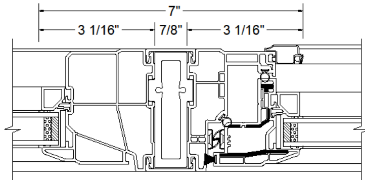
B - FIXED(WITH SASH)/CASEMENT MULLION 7/8" REINFORCEMENT DETAIL
