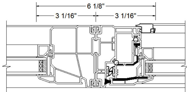
A - FIXED(WITH SASH)/CASEMENT MULLION DETAIL
