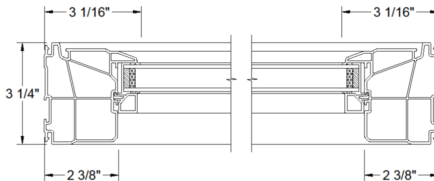
HORIZONTAL SECTION
