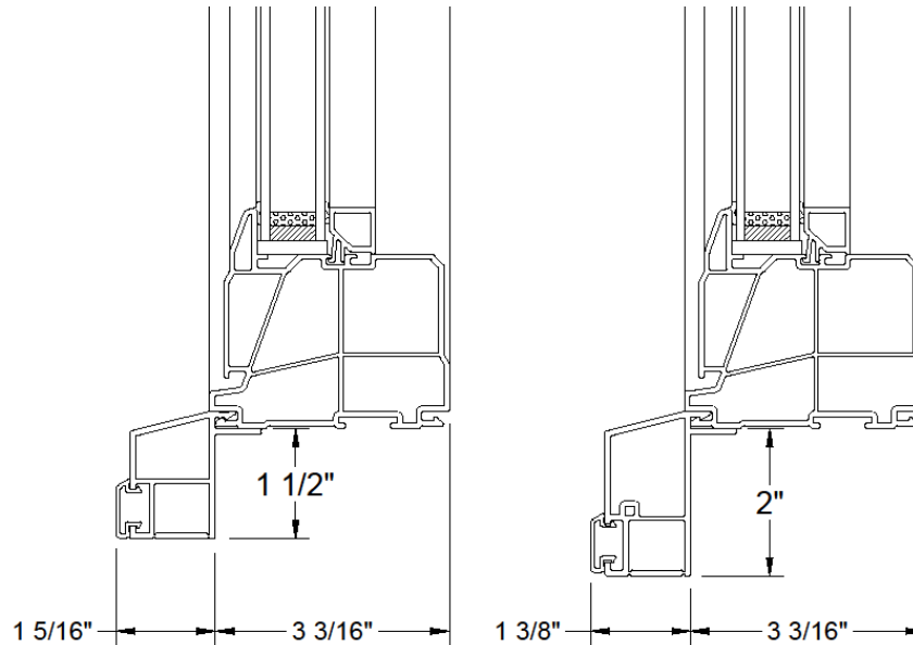
1-1/2" BRICKMOLD WITH CAP
