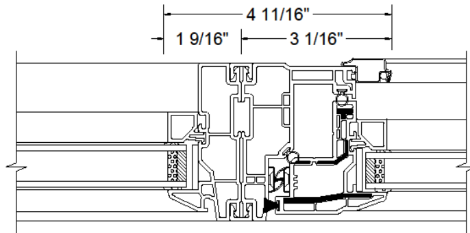
A - FIXED(NO SASH)/CASEMENT MULLION DETAIL
