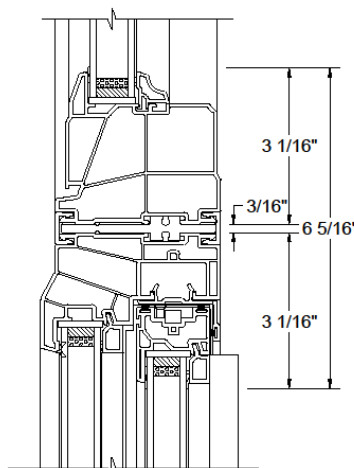
C - FIXED(WITH SASH) OVER SSL MULLION DETAIL
