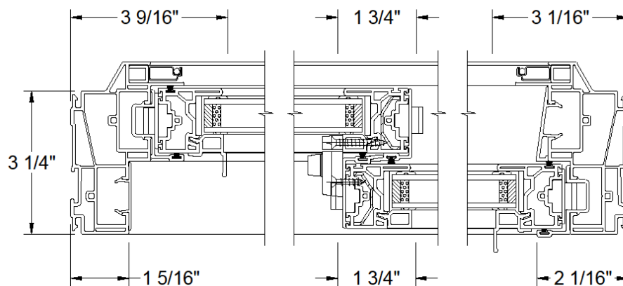
HORIZONTAL SECTION
