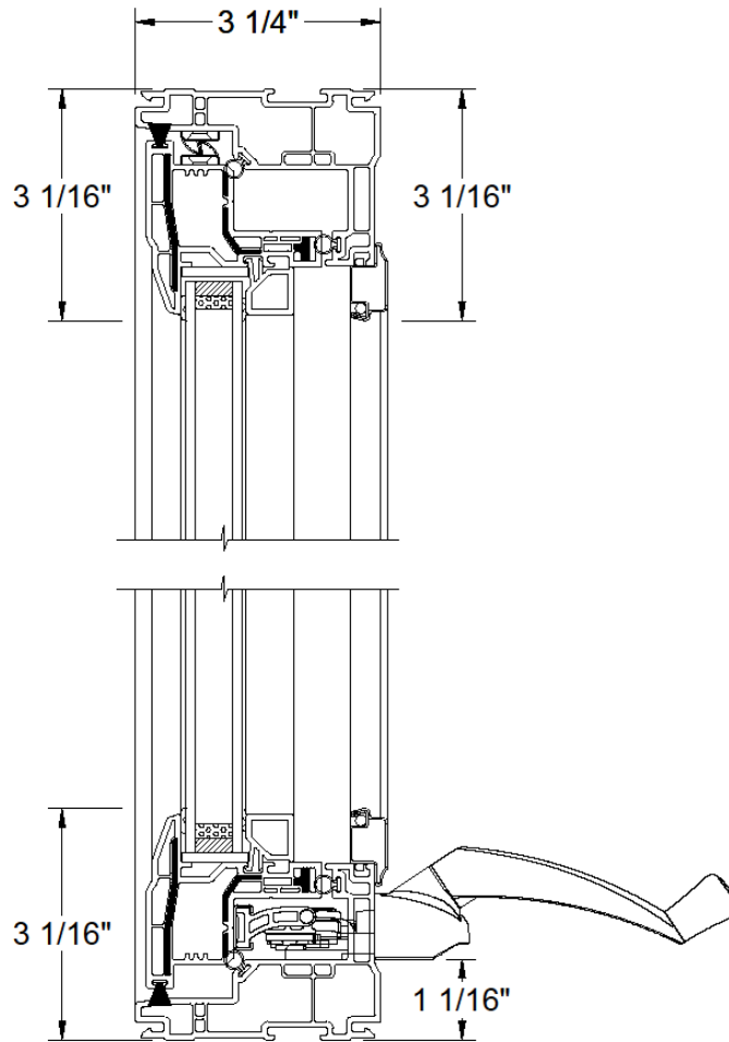
VERTICAL SECTION
