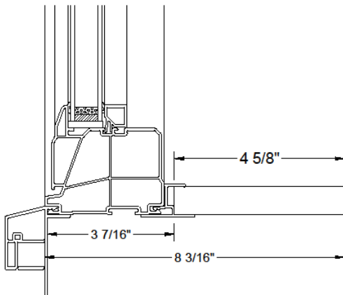
4-5/8" PRIME/VINYL JAMB EXTENSION WITH BRICKMOLD
