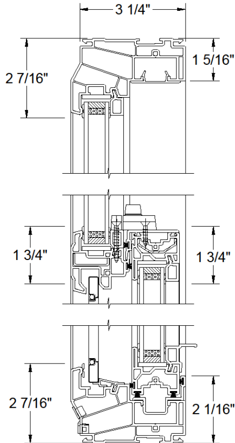
VERTICAL SECTION
