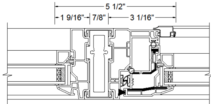
B - FIXED(NO SASH)/CASEMENT MULLION 7/8" REINFORCEMENT DETAIL
