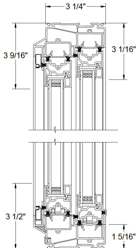
VERTICAL SECTION
