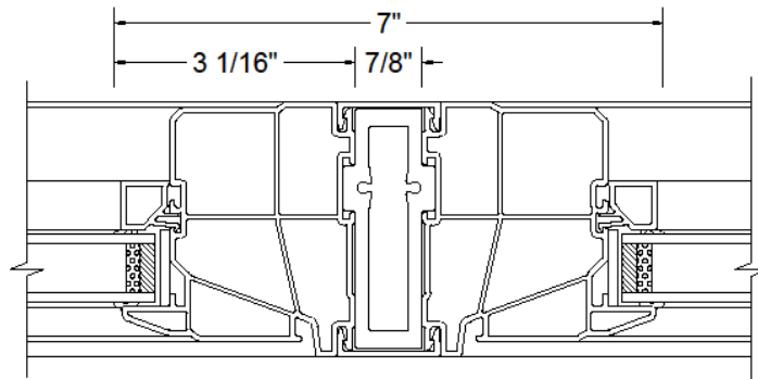
B - FIXED(WITH SASH)/FIXED(WITH SASH) MULLION 7/8" REINFORCEMENT DETAIL
