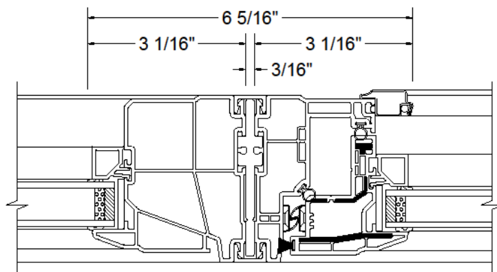
C - FIXED(WITH SASH)/CASEMENT MULLION 3/16" REINFORCEMENT DETAIL
