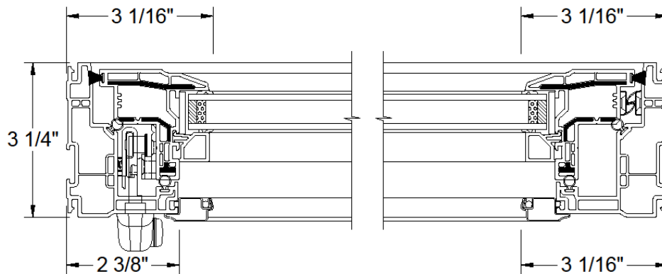
HORIZONTAL SECTION
