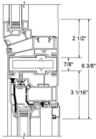
B - FIXED(SINGLE FRAME) OVER AWNING MULLION DETAIL
