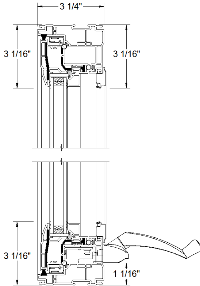
VERTICAL SECTION
