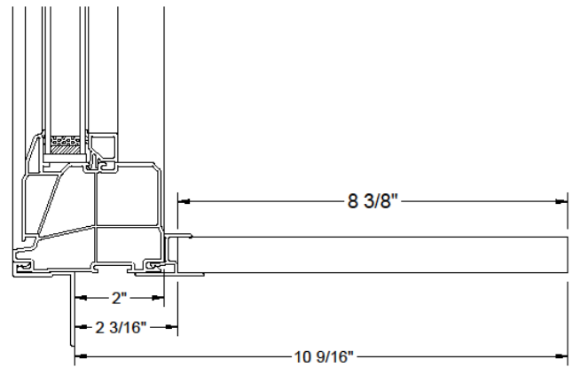
8-3/8" PRIME/VINYL JAMB EXTENSION WITH NAIL FIN
