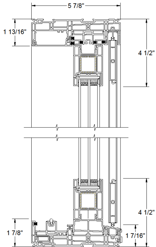
VERTICAL SECTION (FIXED SIDE)
