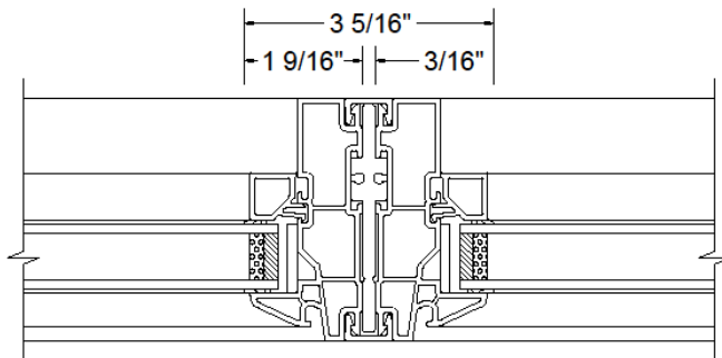
C - FIXED(NO SASH)/FIXED(NO SASH) MULLION 3/16" REINFORCEMENT DETAIL
