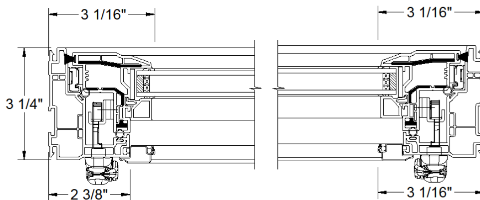
HORIZONTAL SECTION
