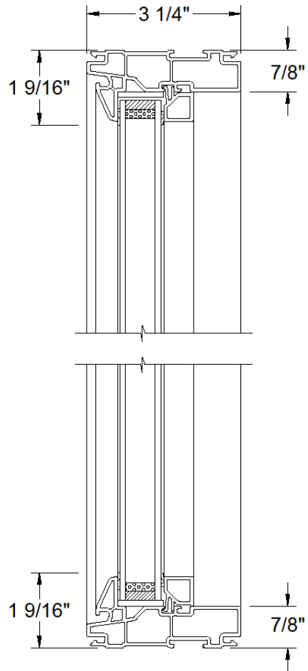
VERTICAL SECTION
