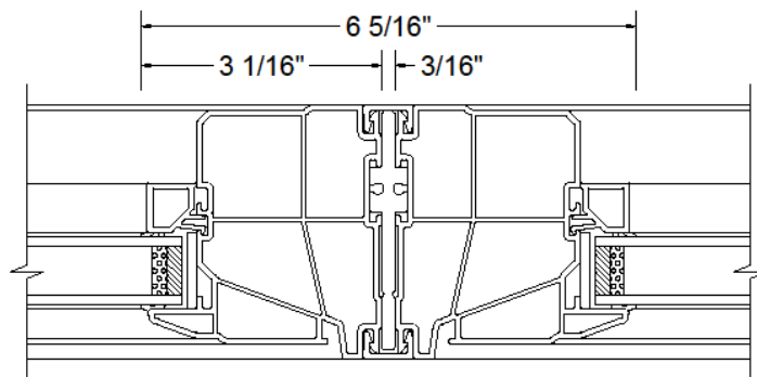
C - FIXED(WITH SASH)/FIXED(WITH SASH) MULLION 3/16" REINFORCEMENT DETAIL
