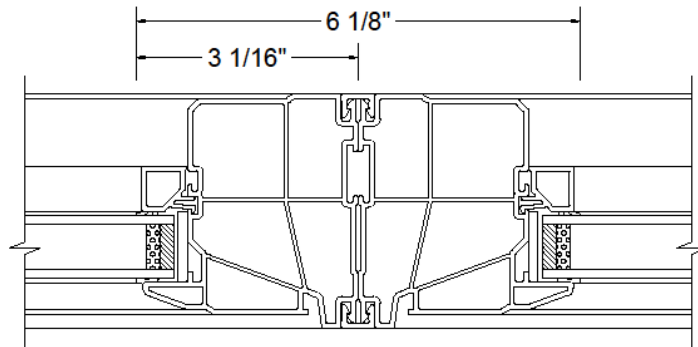
A - FIXED(WITH SASH)/FIXED(WITH SASH) MULLION DETAIL
