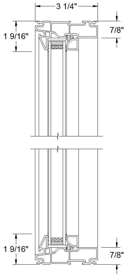
VERTICAL SECTION
