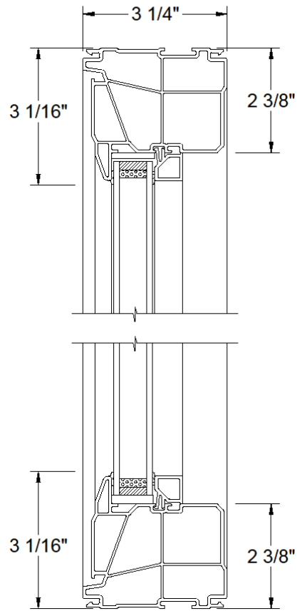
VERTICAL SECTION
