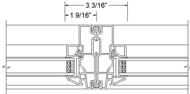
A - FIXED(NO SASH)/FIXED(NO SASH) MULLION DETAIL
