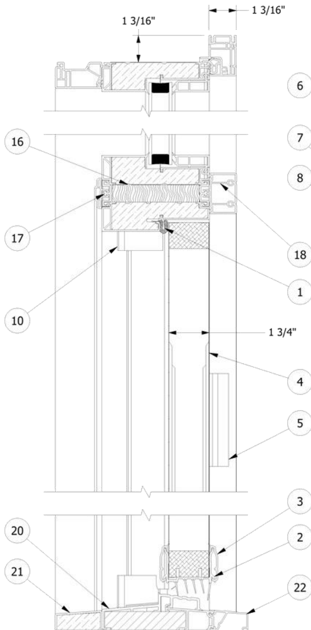
Vertical Section A-A
