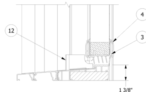
Vertical Section A-A
