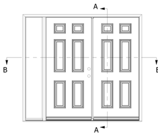
Exterior View LH Active Not to Scale
