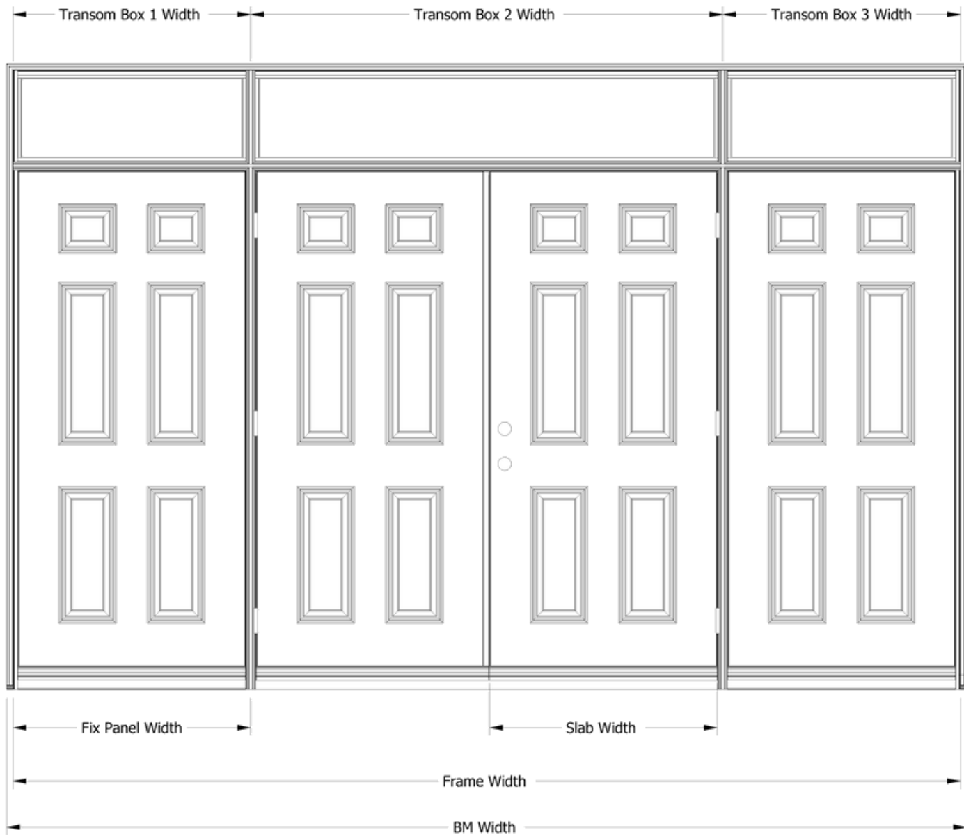
Interior View - Inswing LH Active
