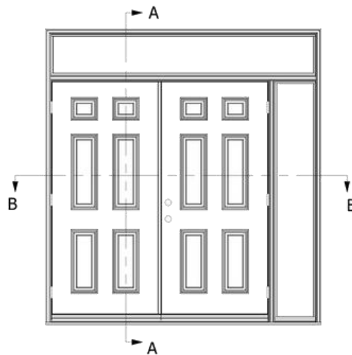
Exterior View OS LH Active Not to Scale
