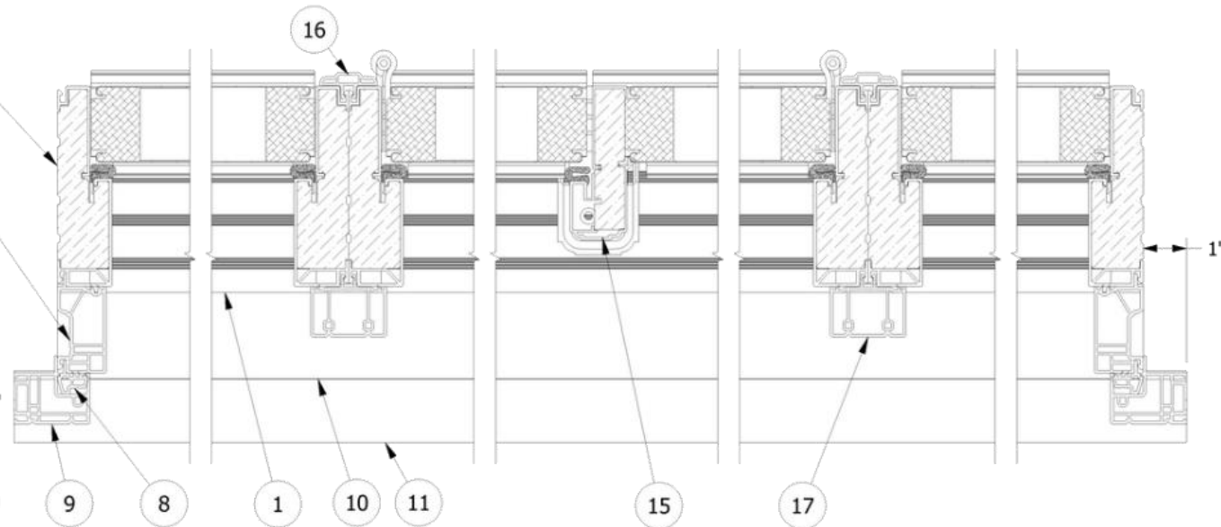
Horizontal Section B-B
