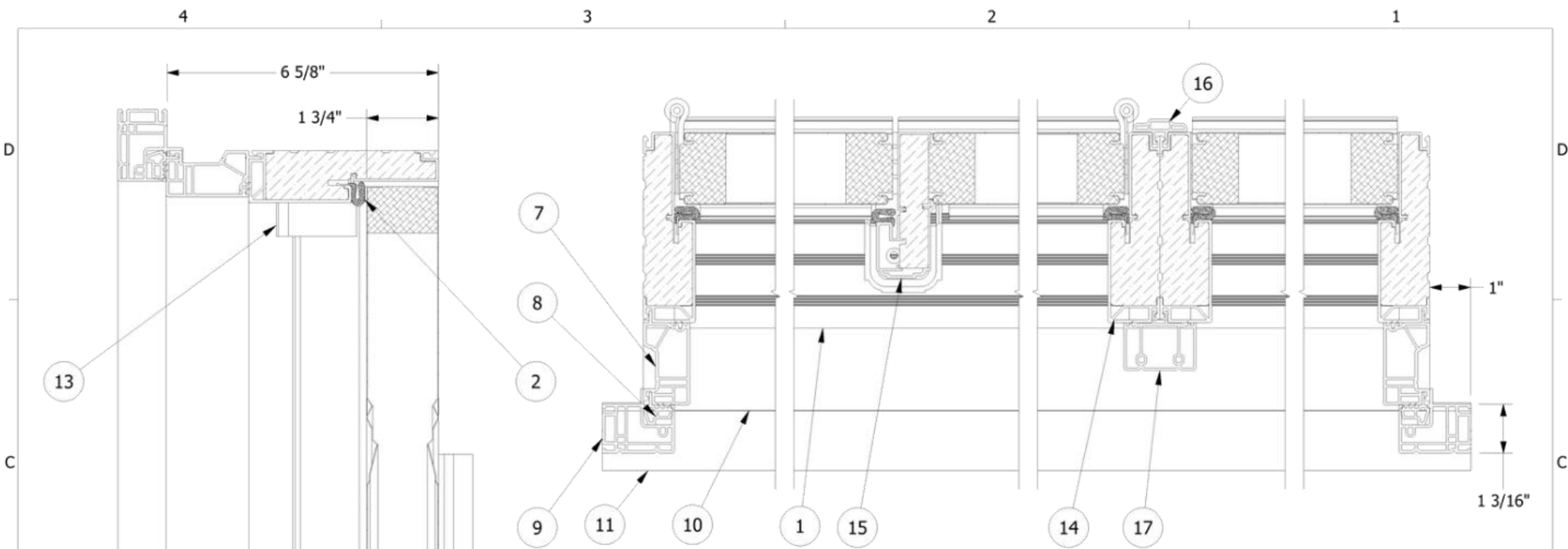
Horizontal Section B-B
