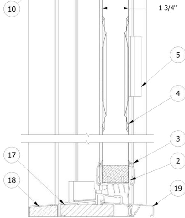
Vertical Section A-A
