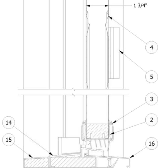
Vertical Section A-A
