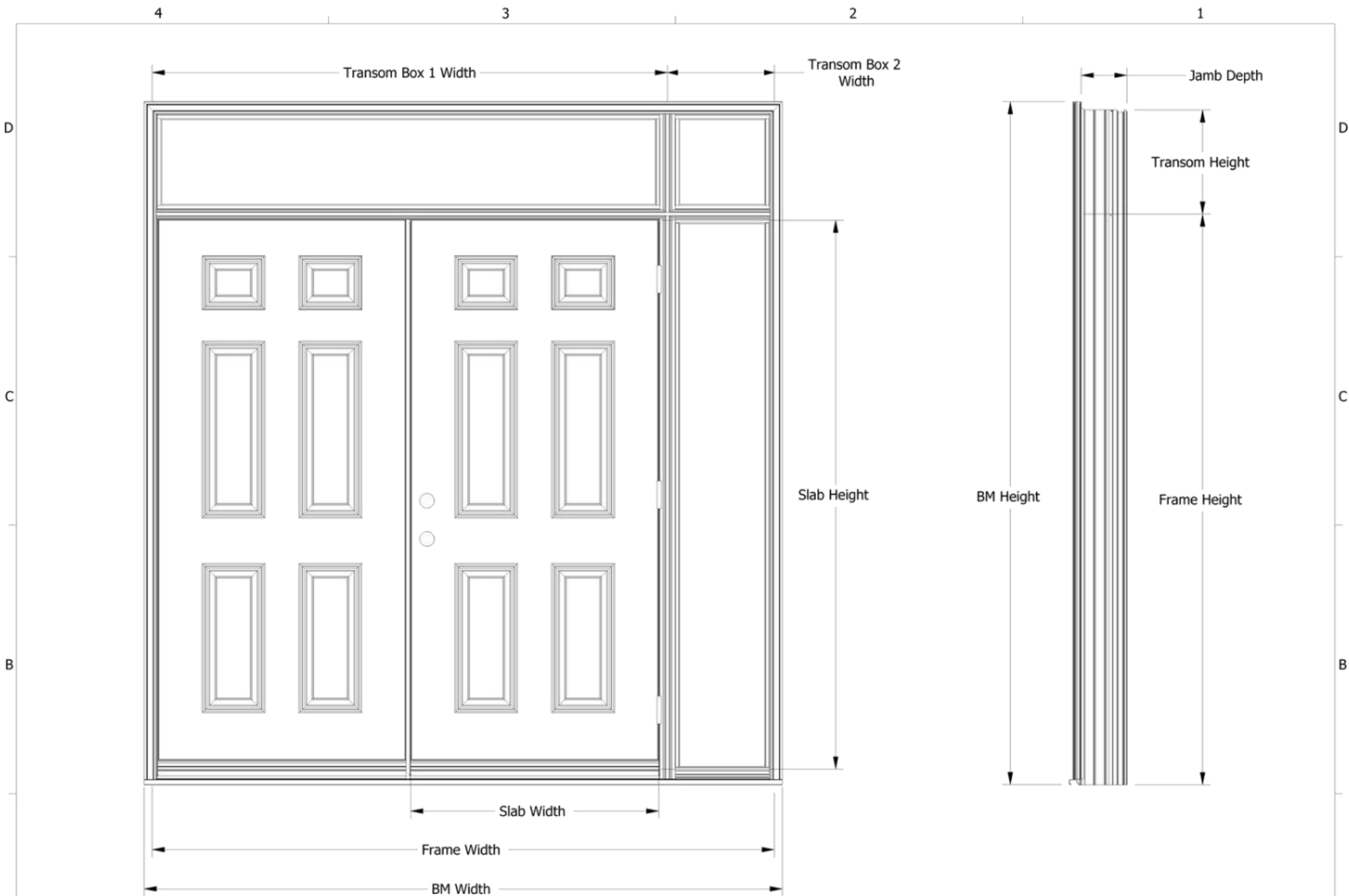
System with Two Box Transom Exterior View - Outswing LH Active
