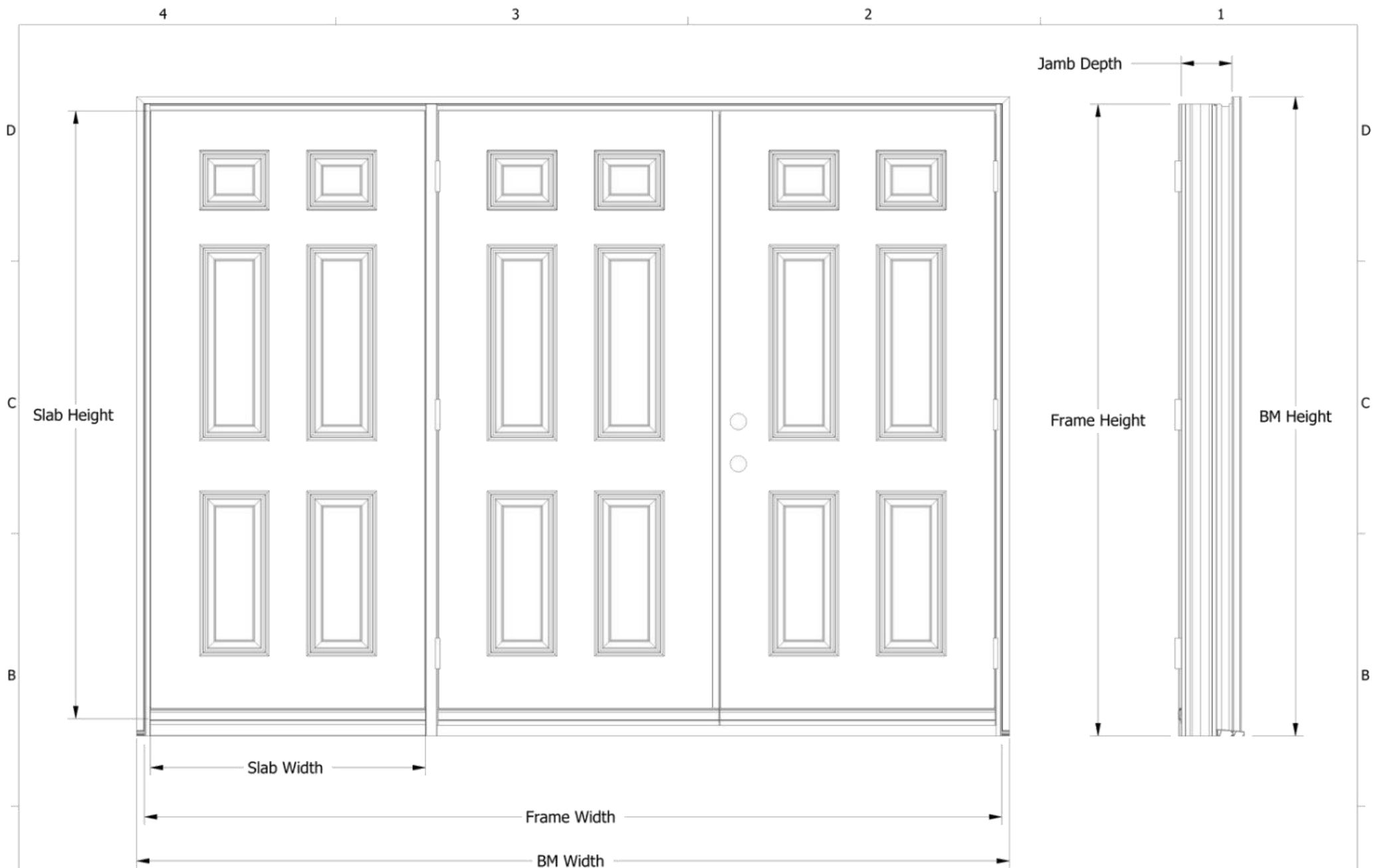
Interior View - Inswing LH
