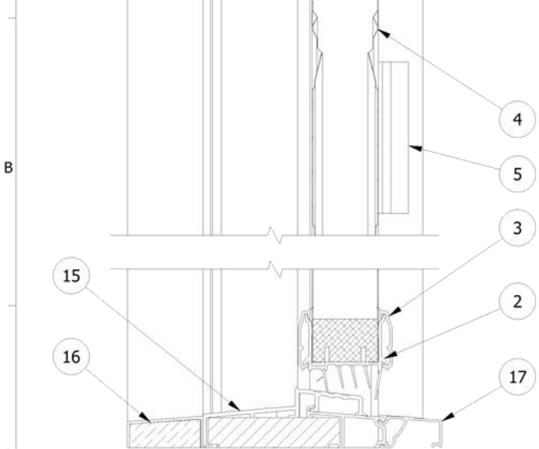
Vertical Section A-A
