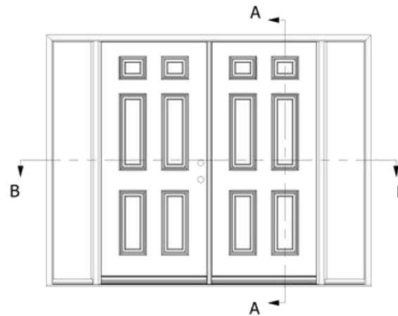
Exterior View LH Active Not to Scale
