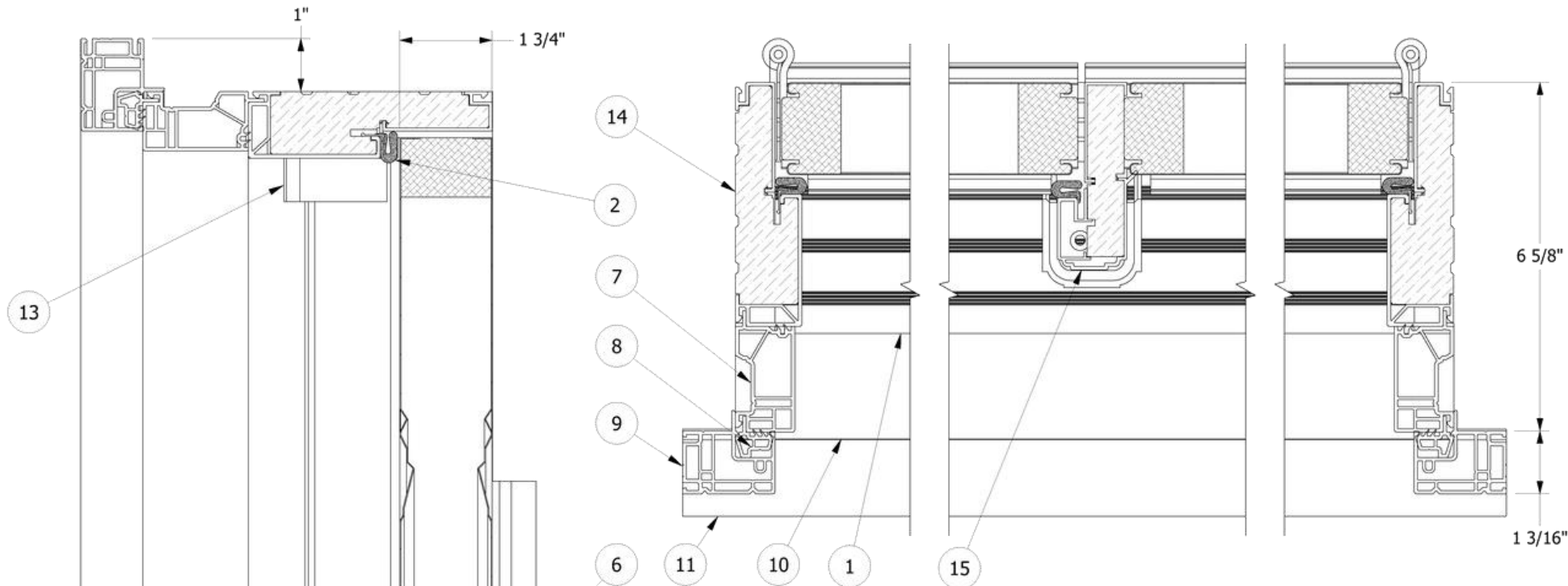
Horizontal Section B-B
