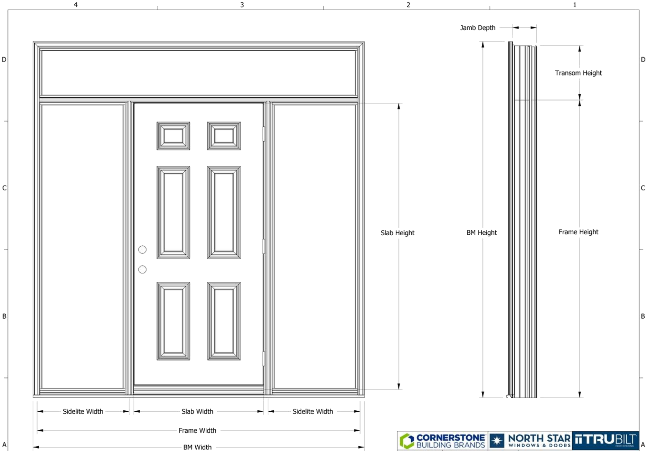
Exterior View - Outswing LH
