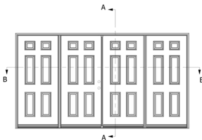
Exterior View LH Active Not to Scale
