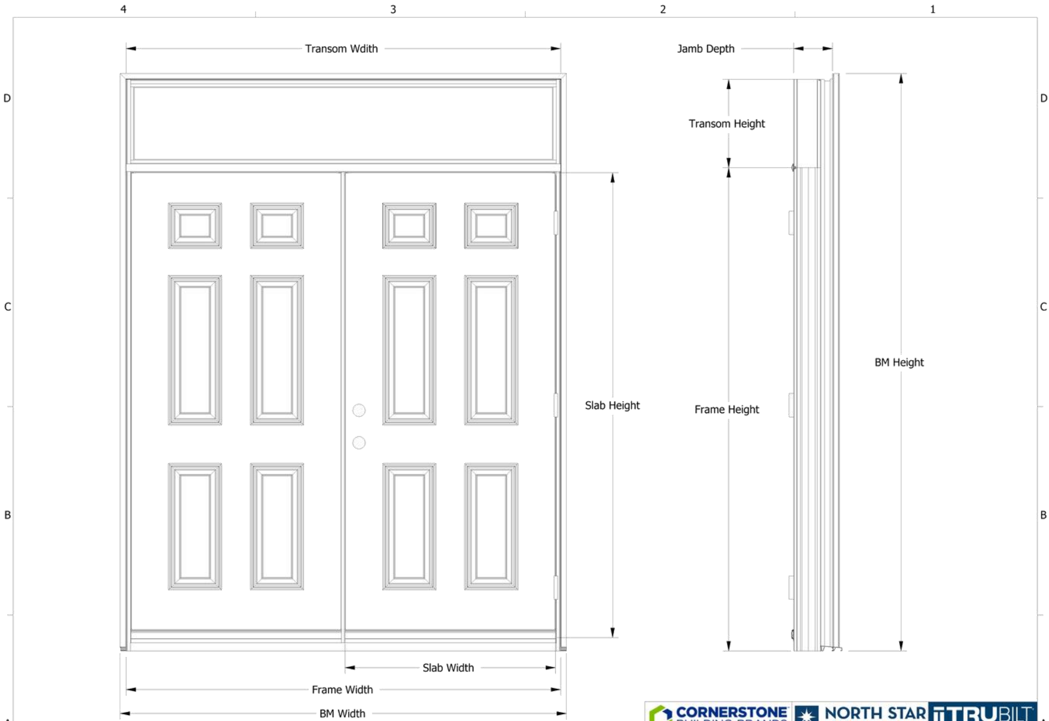
Interior View - Inswing LH Active
