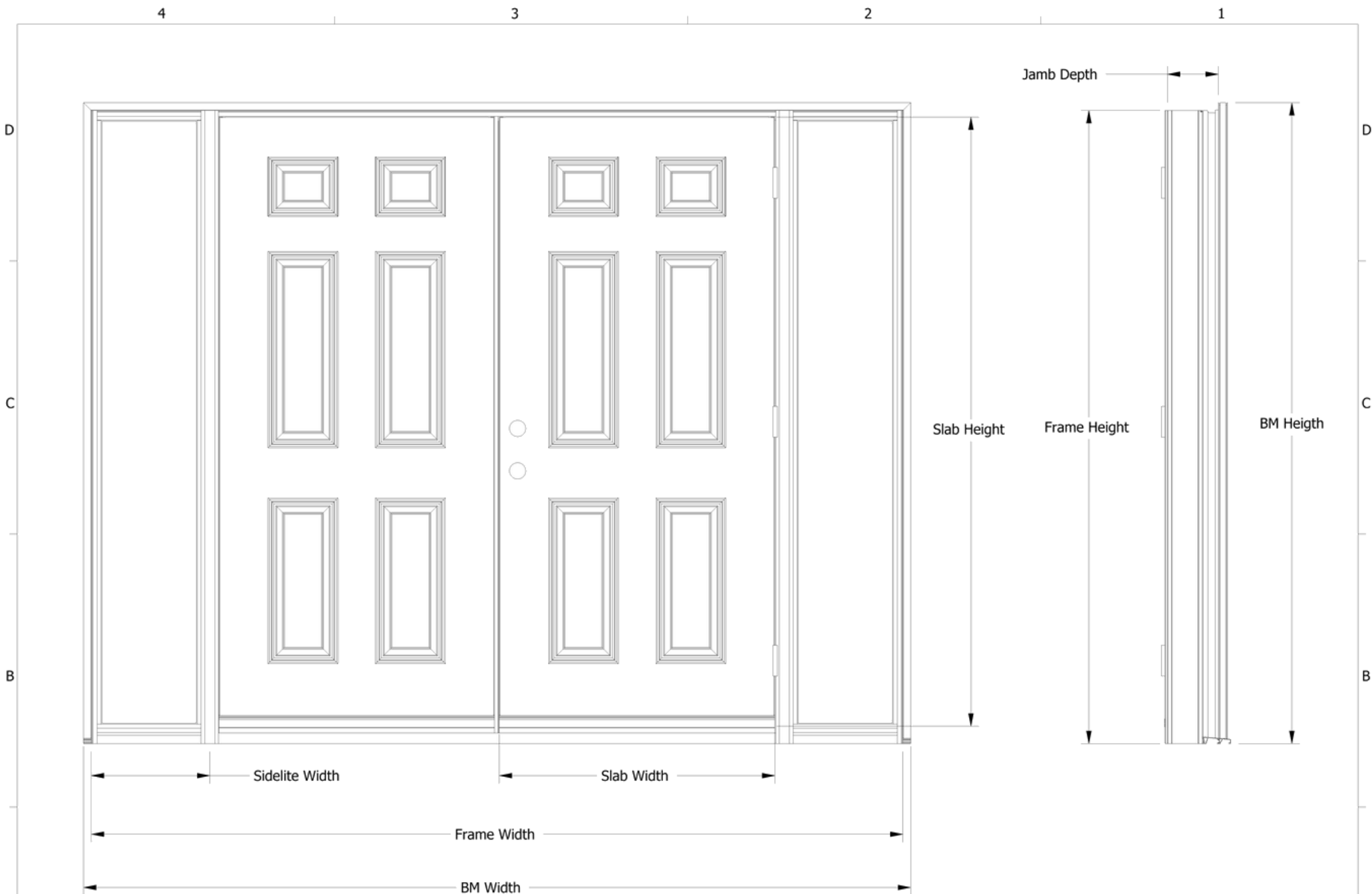
Interior View - Inswing LH Active
