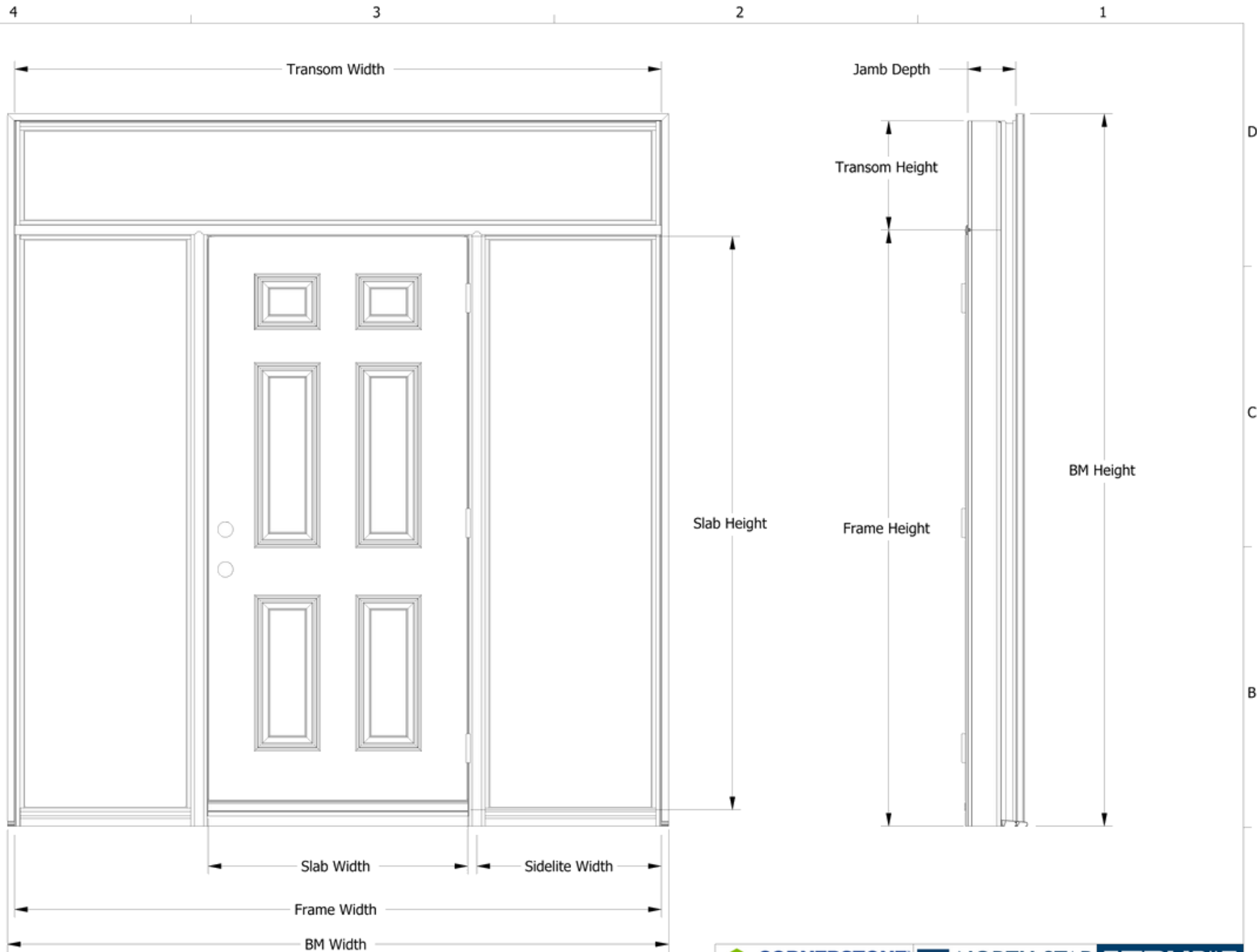
Interior View - Inswing LH
