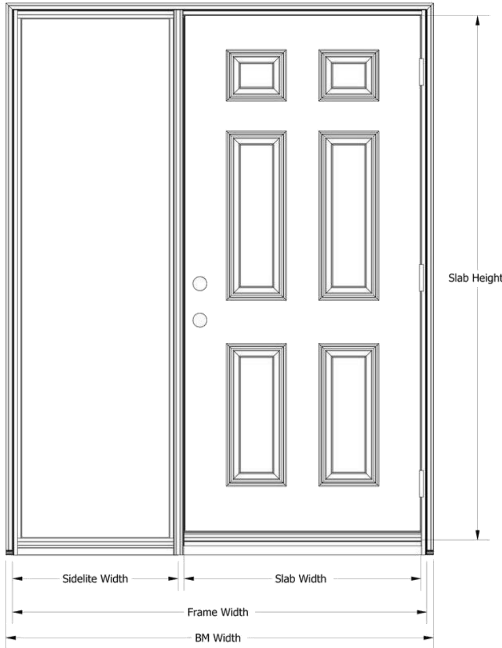
Interior View - Inswing LH
