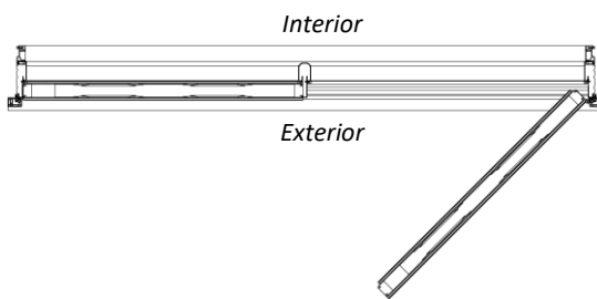
Outswing Left Hand Active*
