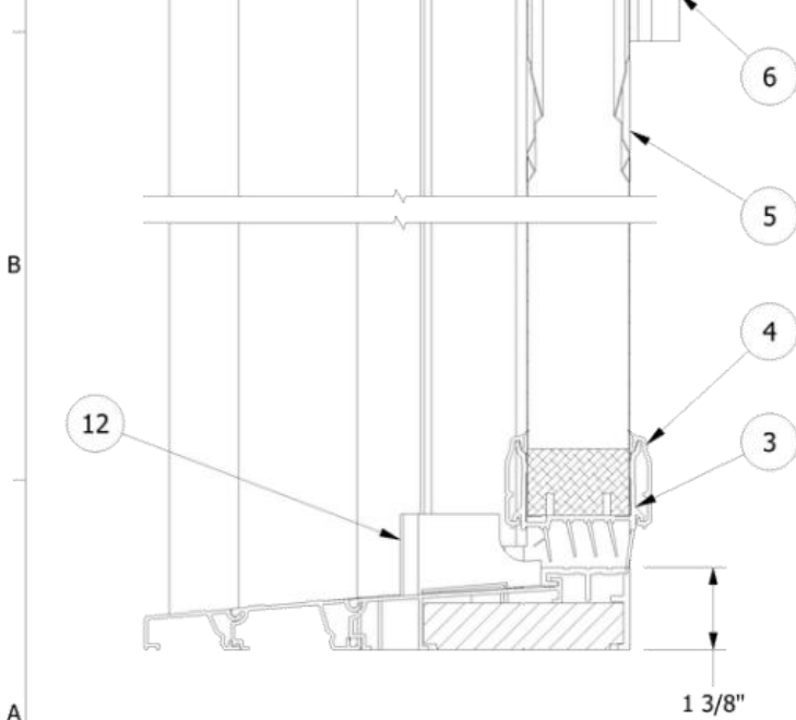
Vertical Section A-A
