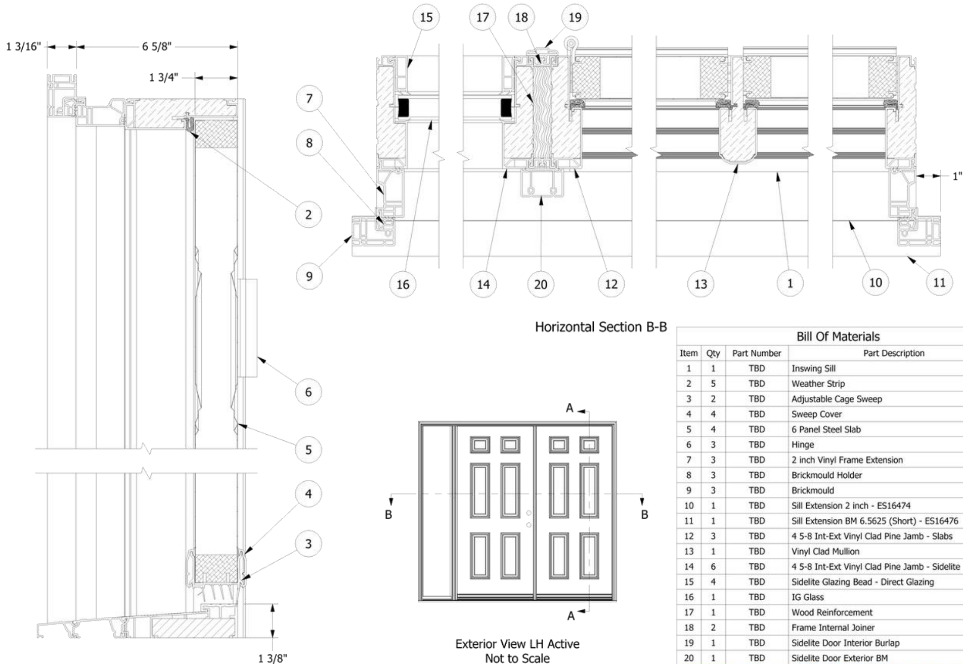
Vertical Section A-A
