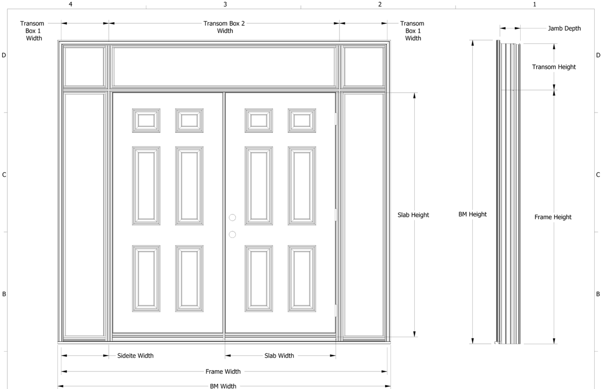
System with Three Box Transom Exterior View - Outswing LH Active
