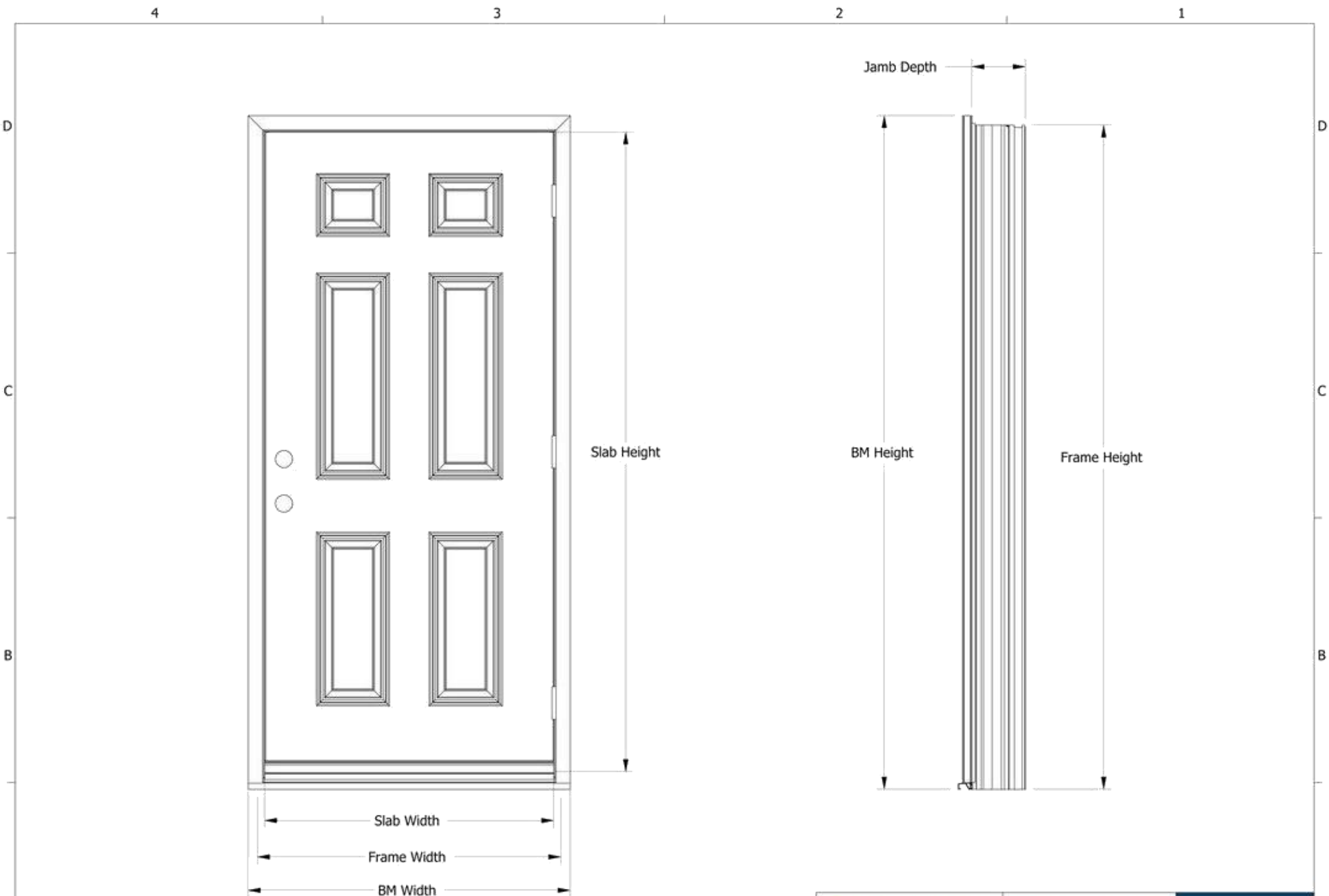
Exterior View - Outswing LH
