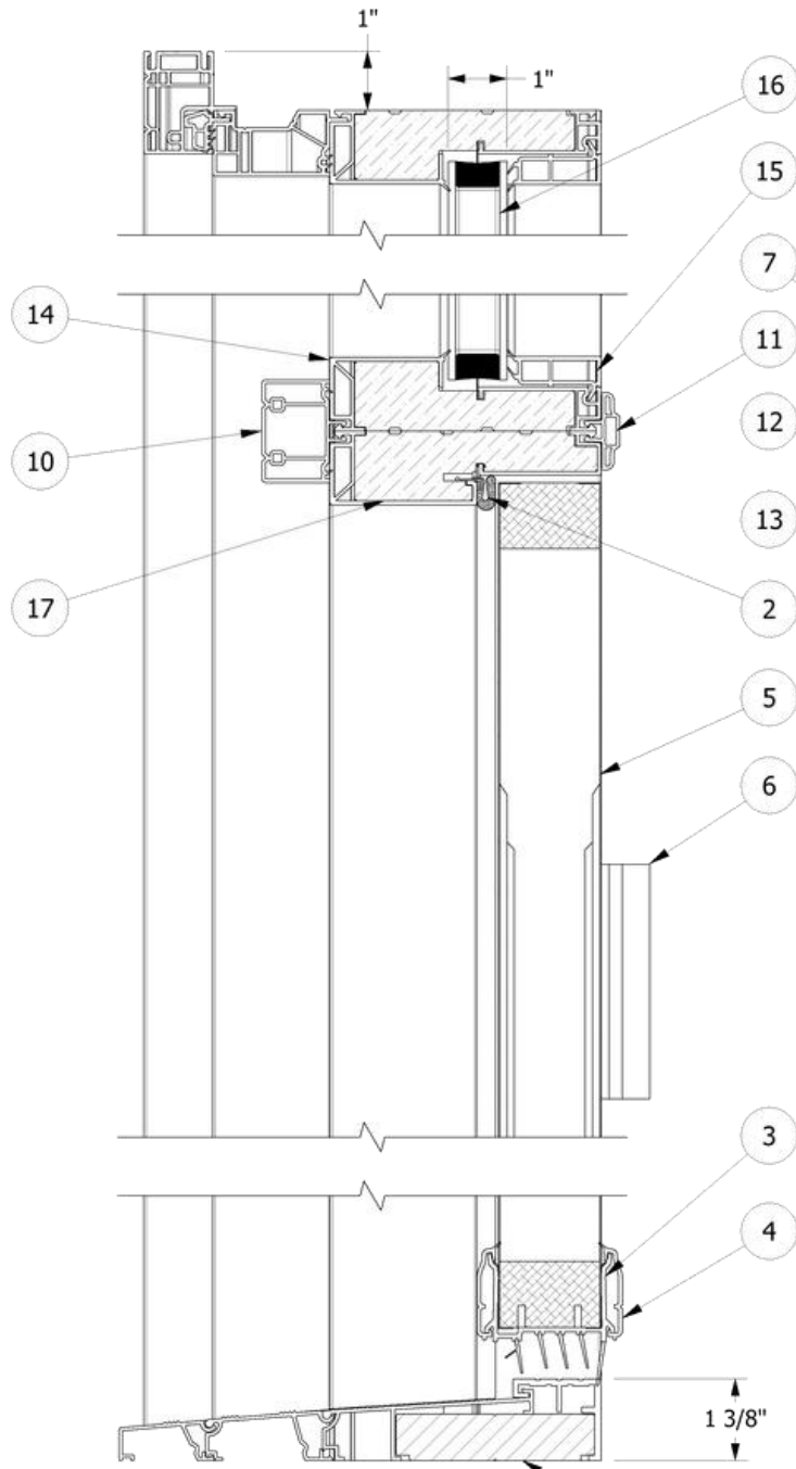
Vertical Section A-A
