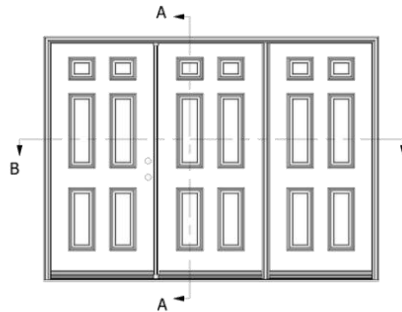
Exterior View LH Active Not to Scale
