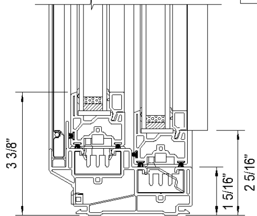
SILL DETAIL
