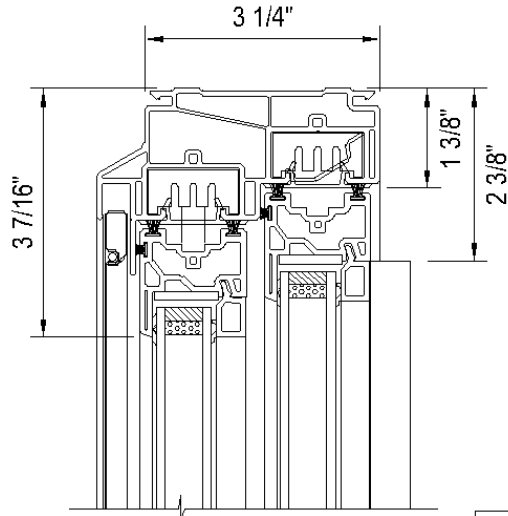
HEAD DETAIL
