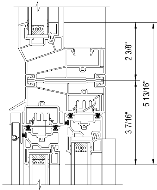
A - PICTURE (SINGLES FRAME) OVER DOUBLE SLIDER TILT MULLION DETAIL
