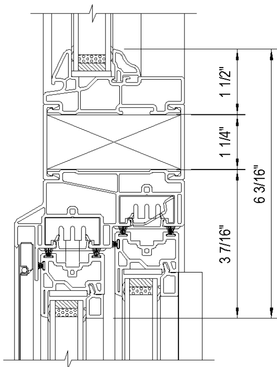
B - FIXED OVER DOUBLE SLIDER TILT MULLION REINFORCEMENT DETAIL
