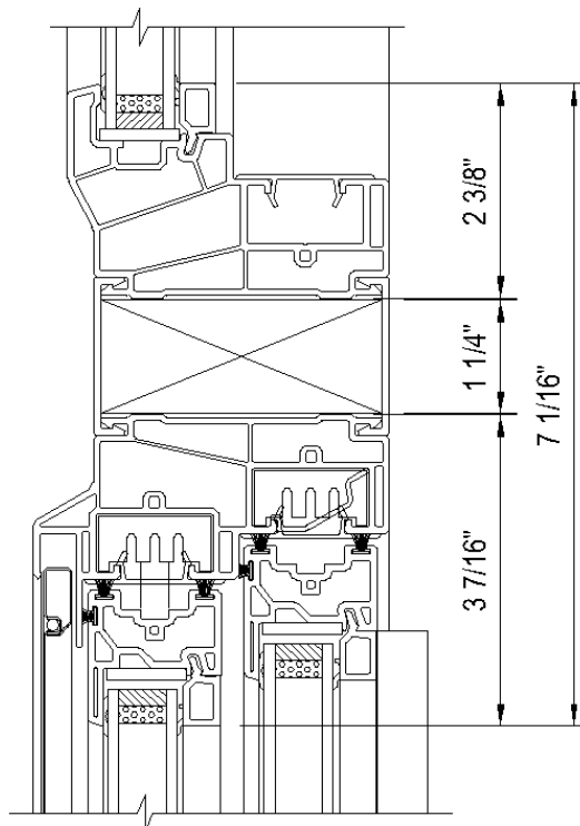
B - PICTURE (SINGLES FRAME) OVER DOUBLE SLIDER TILT MULLION REINFORCEMENT DETAIL
