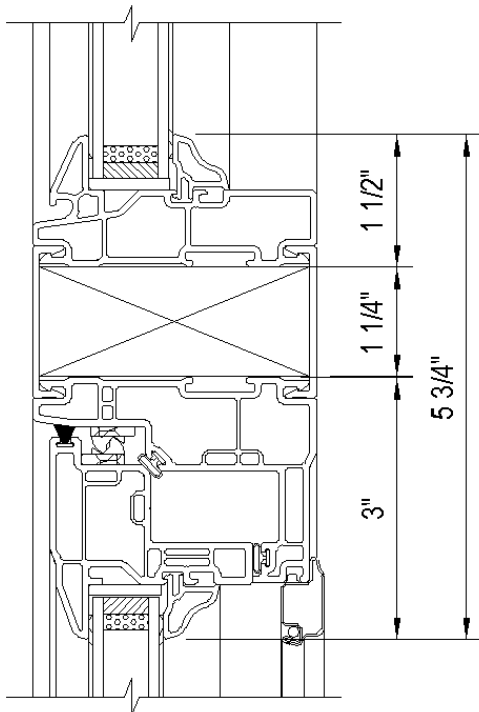
B - FIXED OVER AWNING MULLION REINFORCEMENT DETAIL
