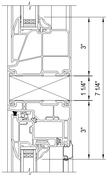
B - PICTURE OVER AWNING MULLION REINFORCEMENT DETAIL
