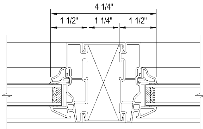
B - FIXED/FIXED MULLION REINFORCEMENT DETAIL
