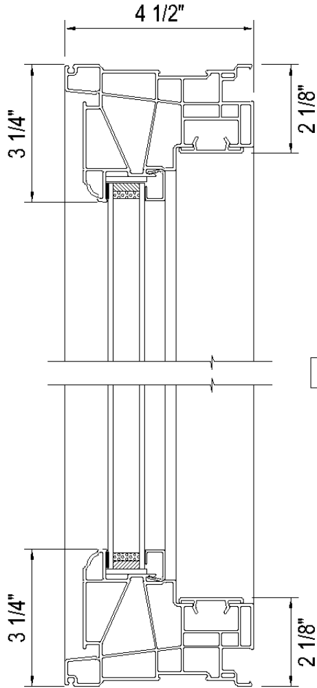
SILL DETAIL
