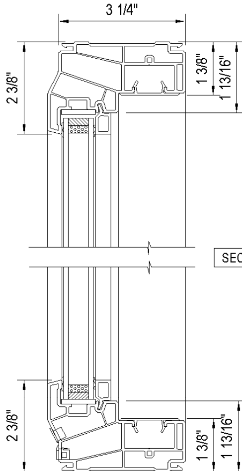
HEAD DETAIL
