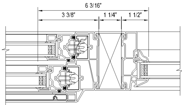
C - DOUBLE HUNG TILT/FIXED MULLION REINFORCEMENT DETAIL
