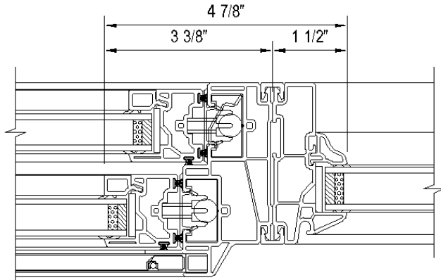
A - DOUBLE HUNG TILT/FIXED MULLION DETAIL
