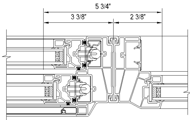
B - DOUBLE HUNG TILT/PICTURE (SINGLES FRAME) MULLION DETAIL
