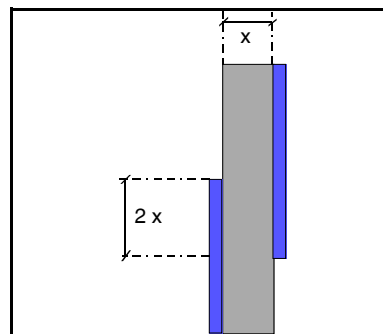
Figure 5-3 Minimum Permissible Insulation Overlap
